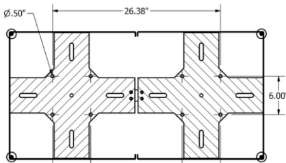
SURFACE MOUNT
